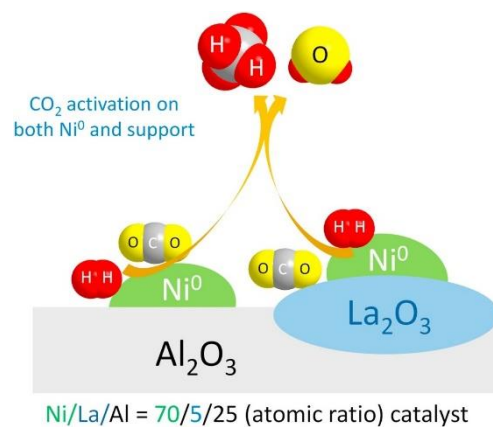
Scheme 1. Proposed mechanism of CO 2 activation and methanation on NiLaAl catalyst via bicarbonate and bidentate formate intermediate pathway.
