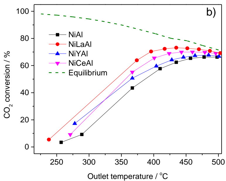
Figure 6. Increment of temperature ( T_{\max} - T_{\text{oven}} ) a) and \text{CO}_2 conversion versus outlet temperature b) during the catalytic test at different temperatures. Total flow rate 240 \text{ ml min}^{-1} , \text{CO}_2/\text{H}_2/\text{N}_2 = 1/4/1 v/v, 30 \text{ mg} catalyst diluted in 470 \text{ mg} quartz, 480 \text{ L g}^{-1} \text{ h}^{-1} .
