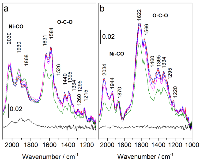
Figure 11. In situ DRIFTS measurements (absorbance mode) of CO 2 adsorption at 200 °C on: a) NiAl and b) NiLaAl catalysts. The first six measurements with increasing of exposure time in CO 2 stream are shown.
