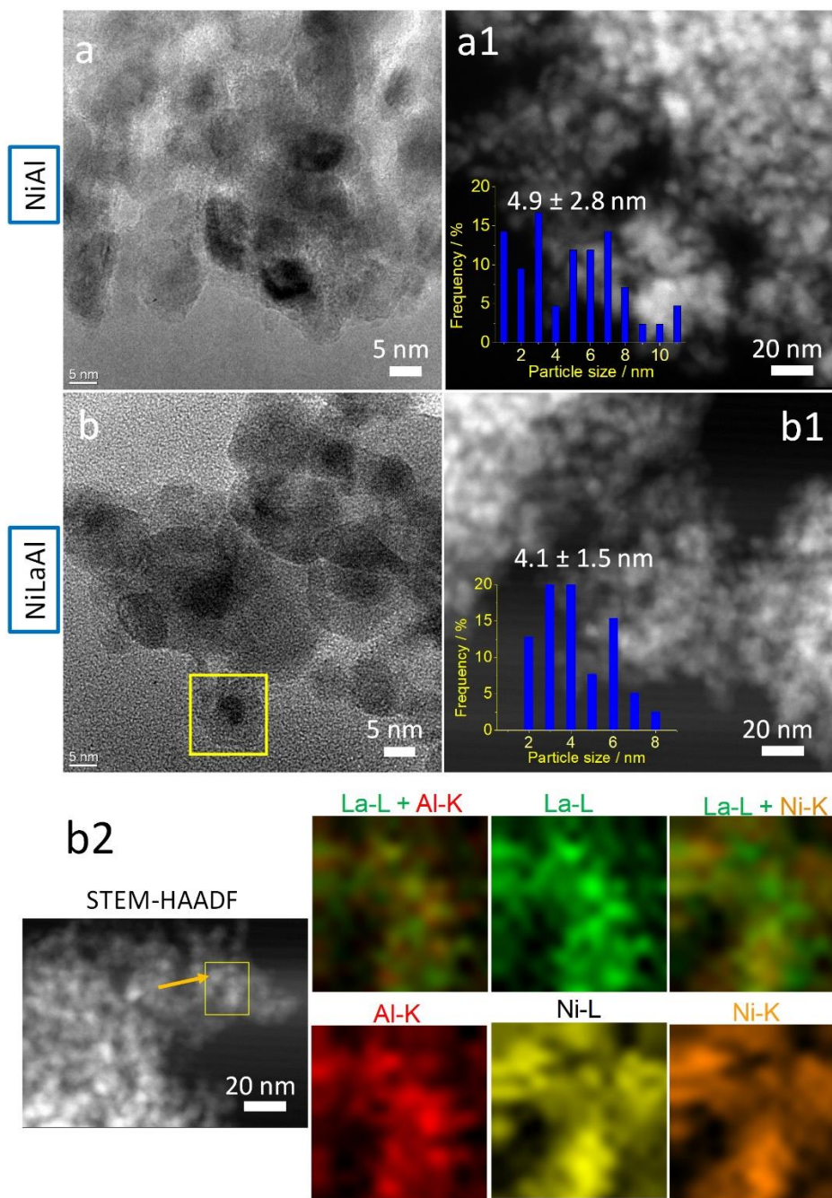
Figure 9. HRTEM images (a, b) and STEM images (a1, b1) and Ni particle size distribution (insets of Fig. a1, b1) of NiAl and NiLaAl used catalysts: a, a1) NiAl; b, b1) NiLaAl. Figure b2 shows elemental distribution in used NiLaAl catalyst after long-term stability test: The left image is from STEM-HAADF and the particle indicated by the arrow is around 6 nm which is a reference point for dimension of the elemental distribution maps on the right.
