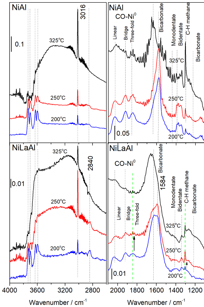
Figure 12. In situ DRIFTS measurements (absorbance mode) in mixture of CO 2 /H 2 /N 2 = 1/4/1 v/v at 200, 250 and 325 °C on NiAl and NiLaAl.
