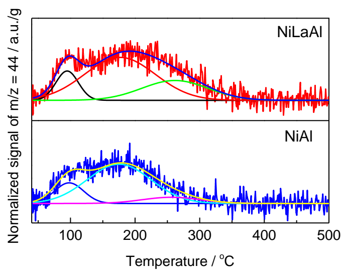
Figure 4. CO 2 -TPD profiles of NiAl and NiLaAl catalysts derived from mass number m/z = 44 of mass spectrometer. The y-axis scale is the same for both catalysts. Detailed information of the deconvoluted peaks is summarized in Table 3.
