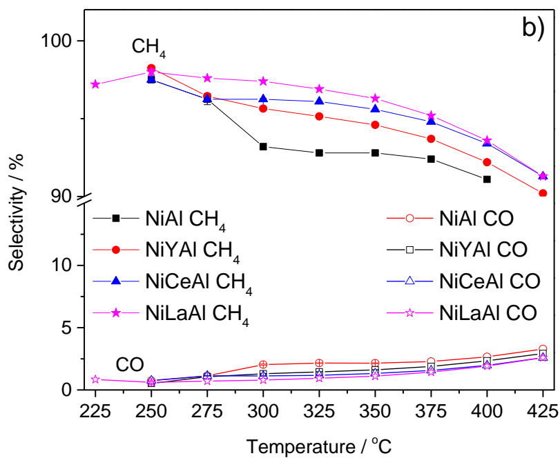
Figure 5. CO 2 conversion (a) and Selectivity in CH 4 and CO (b) on NiAl and NiXAl catalysts. Total flow rate 240 ml min -1 , CO 2 /H 2 /N 2 = 1/4/1 v/v, 30 mg catalyst diluted in 470 mg quartz, 480 L g -1 h -1 .
