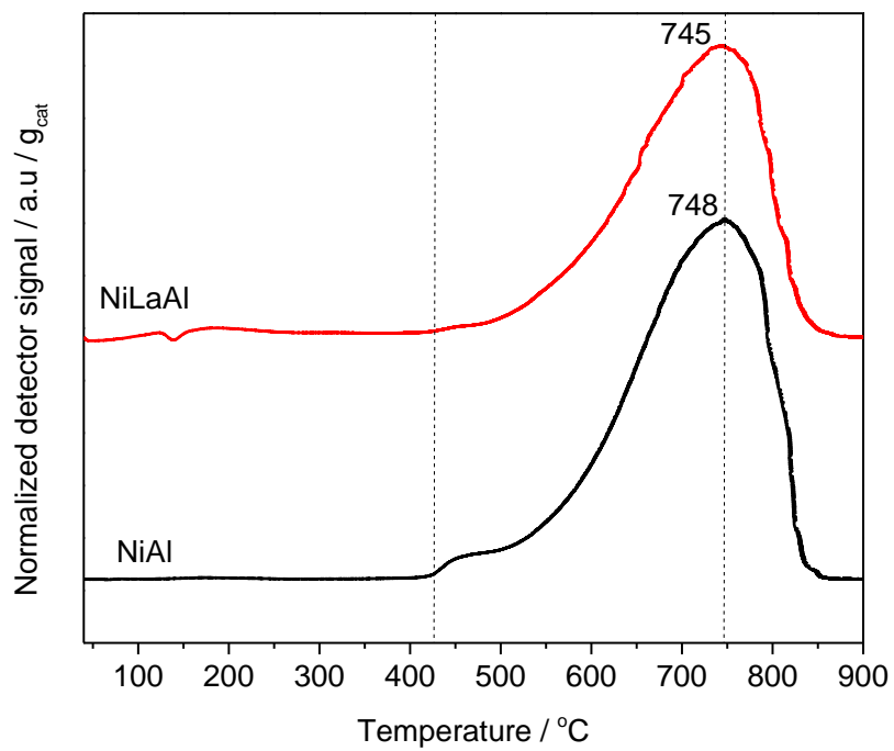
Figure 3. H 2 -TPR profiles of NiAl and NiLaAl catalysts.
