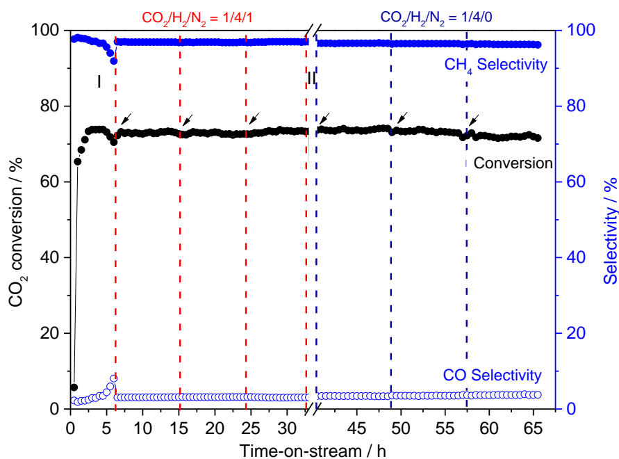
Figure 7. Stability test of CO 2 methanation on NiLaAl catalyst at 325 °C. The first 6 h is the test at different oven temperature. Total flow rate 240 ml min -1 , 30 mg catalyst diluted in 470 mg quartz, 480 L g -1 h -1 . Arrows indicate shut-down (to room temperature) and start-up in N 2 flow.
