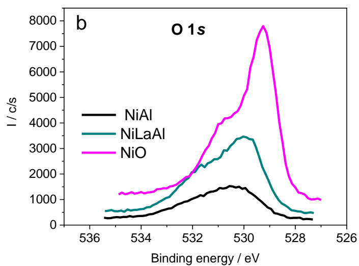
Figure 2. XPS of NiAl and NiLaAl catalysts: a) Ni 2p_{3/2} , b) O 1s (the XPS of NiO is also included).
